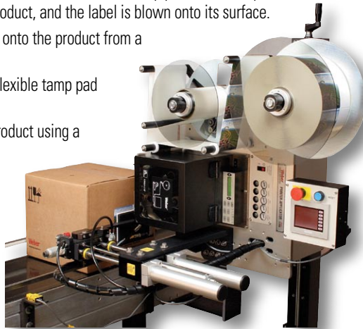
Twin-tamp Configuration
